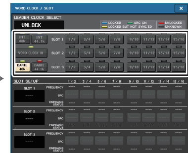
WORD CLOCK/SLOT SETUP 窗口
