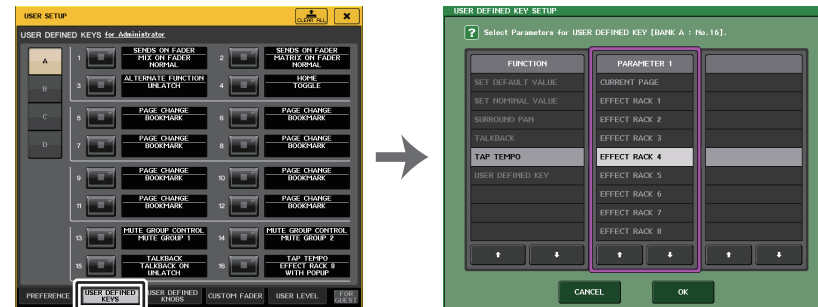
USER SETUP 屏幕 (USER DEFINED KEYS 页面)
